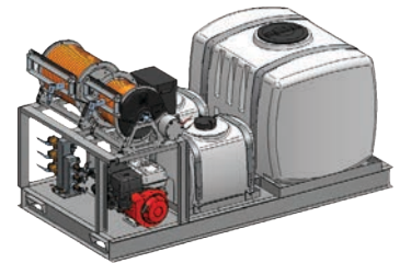
200/30/30 GALLON SKID
